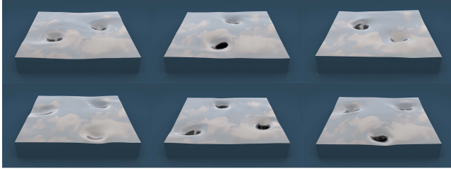
Fig. 7. Interactions of two (top) and three (bottom) parallel vortices on free-surface. The top figures from left to right are frame 200, 300 and 400 of the dual-vortex simulation. The bottom figures from left to right are frame 500, 600, and 700 of the tri-vortex simulation, respectively.
